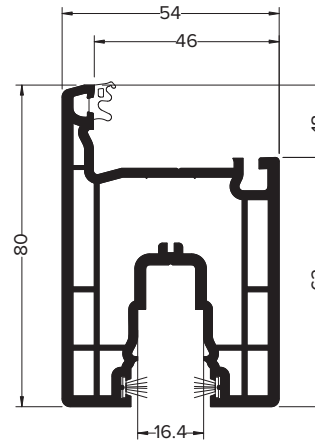
575305 595405 (Foiled) Reinforcement 34.5 x 40.8 DOOR SASH
