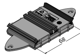
375302 ANTI-LIFT BLOCK
