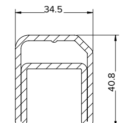
357833 REINFORCEMENT 34.1 X 40.8 X 2.5MM
