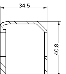
361488 REINFORCEMENT 34.1 X 40.8 X 2MM
